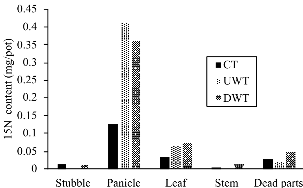
Fig. (5). 15 N content for the three different water treatments during harvest.
