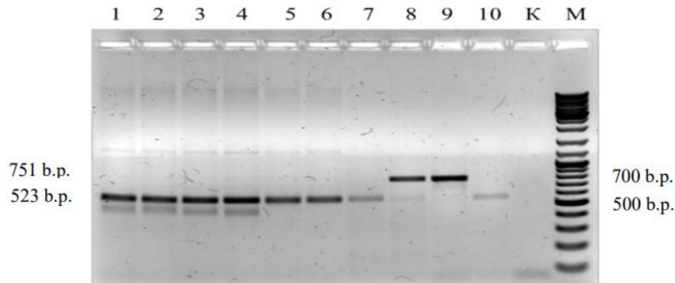
Fig. (3). Electrophoregram of PCR results using the marker cssjfr5 : 1, 2 – ‘Nataalka’, 3, 4 – ‘Zolotokolosa’, 5, 6 – ‘Pivna’, 7 – ‘Kievskaya-Ostistaya’, 10 – ‘Lasunya’. Lanes 1-7, 10 - samples of wheat type Lr34(-) ; 8, 9 – ‘Volodarka’, 8-9 - wheat variety Lr34(+) ; K - negative control (without DNA); M - GeneRuler™ DNA Ladder Mix.
