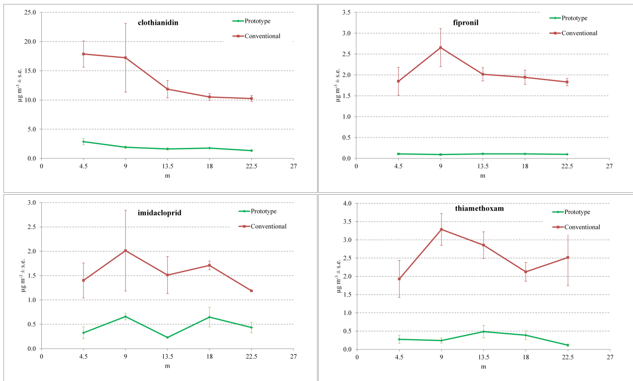
Fig. (3). Comparison between drift values in the sampling area obtained with the conventional drill and the prototype. Values are expressed in terms of air concentrations ( \mu\text{g m}^{-3} \pm \text{standard error} ).
